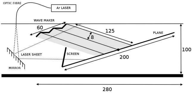
FIG. 2: Sketch of the vertical cross-section of the experimental setup. The sinusoidal thick line on the top left indicates the position of the oscillating paddle, while the grey region defines the incident beam impinging on the sloping glass plane. The optic fibre, indicated by the solid line on the left, shines a laser light which is reflected on the underwater 45 degree mirror, making a thin vertical laser sheet necessary for the PIV measurements. Finally, the dashed line shows the position of the screen which avoids the propagation toward the glass plate of harmonics also generated by the paddle. A slit in the screen allows the laser sheet to pass through. All distances are in centimeter.
