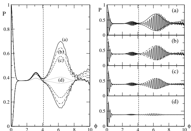
FIG. 8: Influence of dissipation on the spontaneous revivals of the Rabi oscillation signal P = P_{m=J} (as a function of \phi = gt/2\sqrt{\bar{n}} ) for N = 2 atoms. The initial condition is m = 1 (all atoms excited) with \bar{n} = 15 photons. The graph on the left depicts the analytical envelopes P_{\pm}(t) for (a) no dissipation, (b) \gamma^{-1} \simeq 14 ms, (c) \gamma^{-1} \simeq 5 ms and (d) \gamma^{-1} \simeq 1 ms. The right part of the figure presents the associated Rabi oscillation signals obtained from quantum Monte-Carlo simulations (plain lines) as well as the associated analytical envelopes.
