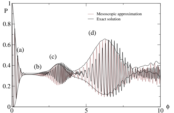
FIG. 5: Spontaneous revivals of the Rabi oscillation signal P = P_{m=J} for N = 3 atoms ( J = 3/2 ), as a function of the dimensionless time \phi = gt/2\sqrt{\bar{n}} . The initial state |m = 3/2\rangle \otimes |\alpha\rangle with an average photon number \bar{n} = |\alpha|^2 = 15 . The signal is computed using the mesoscopic approximation (grey line), its upper and lower envelopes (plain lines) and the exact solution (plain line with rapid oscillations) in the dissipationless case. Letters (a), (b), (c) and (d) refer to the overlaps of cavity field states for each revival depicted in fig. 4. As expected, spontaneous revivals (b) and (c) are symmetric with respect to the flat signal and involve only one rapid frequency, respectively given by 3g\sqrt{\bar{n}} and 2g\sqrt{\bar{n}} .
