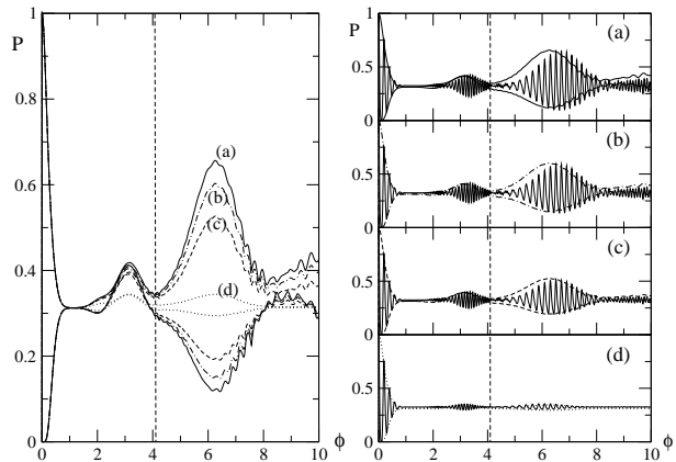
FIG. 9: Influence of dissipation on the spontaneous revivals of the Rabi oscillation signal P = P_{m=J} (as a function of \phi = gt/2\sqrt{\bar{n}} ) for N = 3 atoms. The initial condition is m = 3/2 (all atoms excited) with \bar{n} = 15 photons. The graph on the left depicts the analytical envelopes P_{\pm}(t) for (a) no dissipation, (b) \gamma^{-1} \simeq 14 ms, (c) \gamma^{-1} \simeq 5 ms and (d) \gamma^{-1} \simeq 1 ms. The right part of the figure presents the associated Rabi oscillation signals obtained from quantum Monte-Carlo simulations (plain lines) as well as the associated analytical envelopes.
