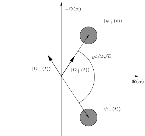
FIG. 1: Schematic evolution of the entangled state for one atom and a mesoscopic coherent state in a cavity for real positive \alpha . The atomic dipole states are represented as arrows. The field coherent states are represented as an uncertainty disk at the tip of the classical amplitude. Each component |D_{\pm}(t)\rangle \otimes |\psi_{\pm}(t)\rangle of the superposition involves an atomic polarization and a field state slowly rotating in the phase plane at velocities \pm g/4\sqrt{\bar{n}} .
