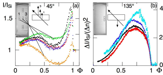
FIG. 4: Intensity scattered by N102 as a function of the condensed fraction \Phi : (a) at 4.47 K and 45^\circ . The signal is normalized by the silica contribution, and corresponds to points at three different depths inside the aerogel. Differences between curves for different depths (and path lengths) are consistent with multiple scattering effects combined with an homogeneous distribution of the liquid clusters within the sample, in contrast to B100 at the same temperature; (b) at 135^\circ , close to the entrance of the laser sheet. The silica contribution I_{Si} has been subtracted, and the result normalized by I_{Si} and the optical contrast squared. The signal is similar at all temperatures, suggesting that the spatial organization of the liquid only depends on \Phi , not on temperature.
