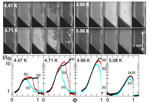
FIG. 3: Images of B100 observed at 45^\circ from the incident laser sheet for helium fractions of 0.1,0.5,0.7,0.9, and 1.0. The curves give the scattered intensity, referred to the empty aerogel situation, for the three spots labelled (a), (b), (c).
