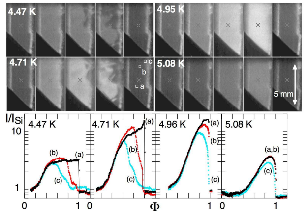
FIG. 3: Images of B100 observed at 45^\circ from the incident laser sheet for helium fractions of 0.1,0.5,0.7,0.9, and 1.0. The curves give the scattered intensity, referred to the empty aerogel situation, for the three spots labelled (a), (b), (c).
