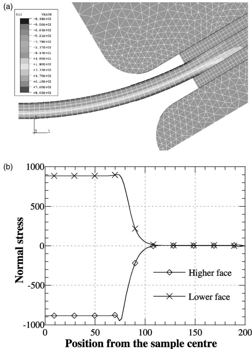
Fig. 8. (a) Normal stress; (b) evolution of the normal stress versus the sample length.
