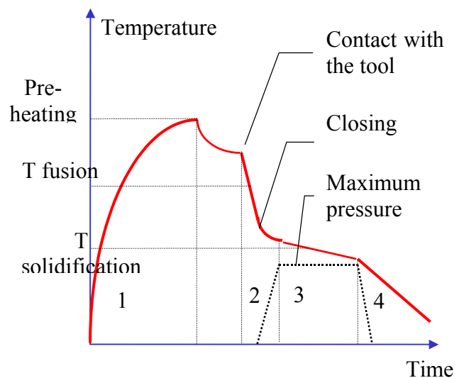
Figure 1: Pressure and temperature during the manufacture 1. Heating of the CFRTP plate 2. Forming with punch and die 3. Reconsolidation phase 4. Release of the final part
