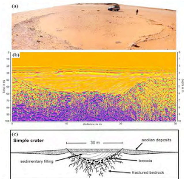
Fig.1: (a) Small-buried crater in GKCF, (b) 270 MHz profile across the buried crater, (c) interpreted model of a simple crater.
