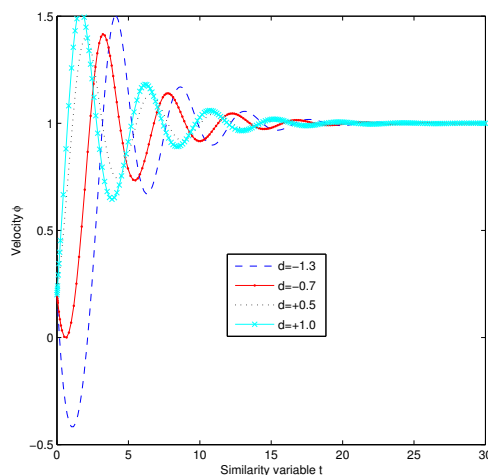
Fig. 4.1 Velocity profiles in terms of d = \theta'(0) for fixed \zeta = 0.2 and \tau = 0.5 .
