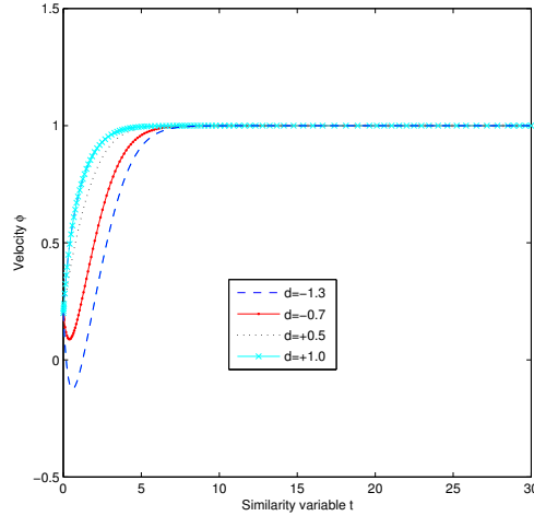
Fig. 4.2 Velocity profiles in terms of d = \theta'(0) for fixed \zeta = 0.2 and \tau = 2.83 .
