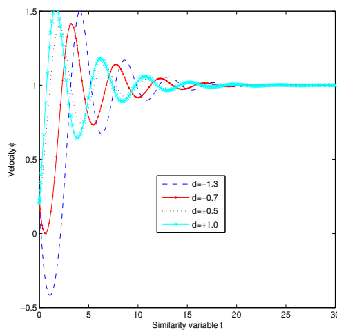
Fig. 4.1 Velocity profiles in terms of d = \theta'(0) for fixed \zeta = 0.2 and \tau = 0.5 .
