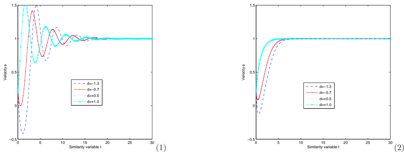
Fig. 1.4 Velocity profiles in terms of d = \theta'(0) for fixed \zeta = 0.2 and \tau = 0.5 (1), and \tau = 2.83 (2).
