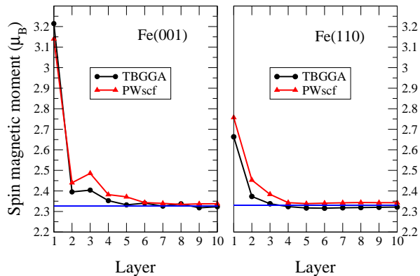
FIG. 6: Variation of the spin magnetic moment (per atom) on successive atomic layers of (001) and (110) slabs (with 20 atomic layers) of bcc Fe obtained from the TBGGA model and PWscf code with GGA. Layer 1 corresponds to the outermost layer and layer 10 to a central layer. The value of the bulk magnetic moment is indicated as a reference.
