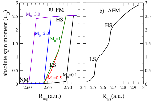
FIG. 2: Variation of the absolute value of the magnetic moment (per atom) for the ferromagnetic (FM) and antiferromagnetic (AFM) states of fcc Fe as a function of the Wigner-Seitz radius R_{WS} , for various input magnetic moments M_0 in \mu_B obtained with TBGGA parameters. LS and HS denote respectively low and high spin states.
