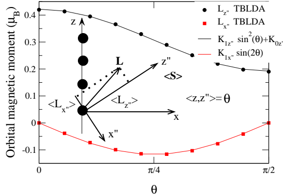
FIG. 13: Variation of the components of the orbital moment relative to the spin framework for a monatomic wire (interatomic distance d = 4.29 a.u.) as a function of the direction of magnetization given by the angle \theta obtained with TBLDA parameters.
