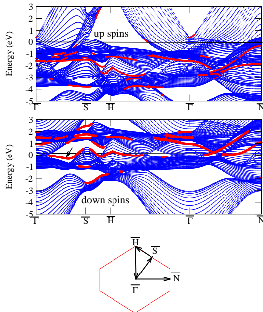
FIG. 5: TBGGA projected band structure for up (top) and down (middle) spins of a 20-layer (110) slab of bcc Fe with the experimental lattice parameter of 2.87\text{\AA} . The energy zero is the Fermi level. Surface or resonant states (i.e., states with more than 60% of their total weight on the first two outer layers) are represented in red and with thicker dots. A characteristic surface state of minority spin is indicated by an arrow. A schematic representation of the surface Brillouin zone and of the path in the reciprocal space is shown at the bottom.
