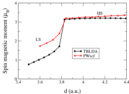
FIG. 10: TBLDA and PWscf spin moment of a monoatomic wire, as a function of the interatomic distance.
