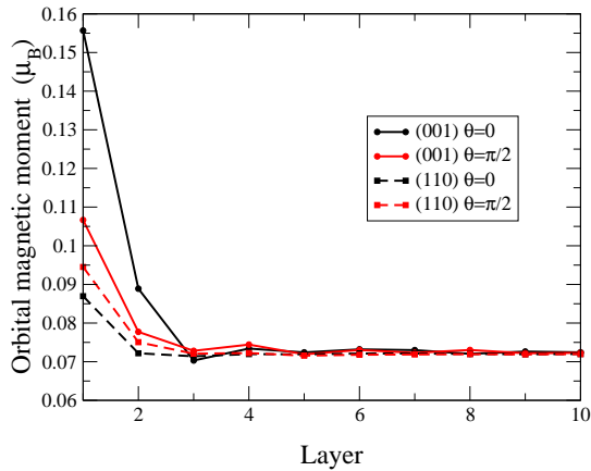
FIG. 8: Variation of the component of the orbital magnetic moment on the magnetization direction (per atom) as a function of the atomic layer in the (110) and (001) slabs (20 layers) for a magnetization perpendicular ( \theta = 0 ) or parallel to the surface ( \theta = \pi/2, \varphi = 0 ).
