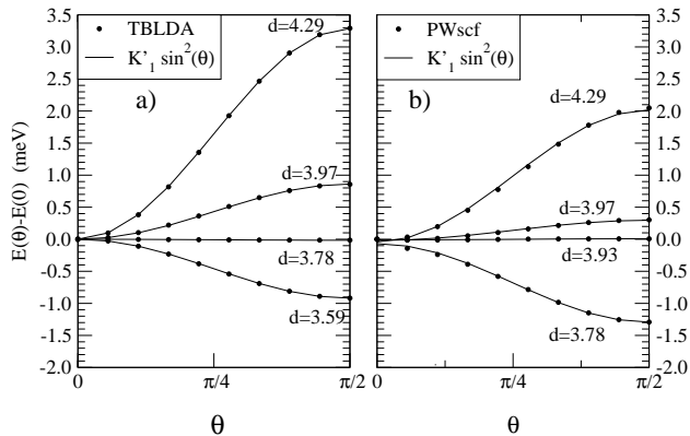
FIG. 12: Variation of the magnetocrystalline anisotropy (per atom) of a monatomic wire as a function of the angle \theta from a TBLDA calculation (left panel) and PWscf calculation (right panel) for various interatomic distances d (in a.u.).
