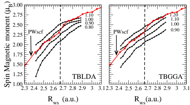
FIG. 1: Variation of the absolute value of the spin magnetic moment (per atom) of bcc Fe as a function of the Wigner-Seitz radius R_{WS} for the values of the Stoner parameter I_{dd'} (in eV) given on each curve. Left and right panels correspond to TBLDA and TBGGA calculations, respectively, compared to PWscf calculations in GGA. The dashed vertical line gives the experimental Wigner-Seitz radius at equilibrium.
