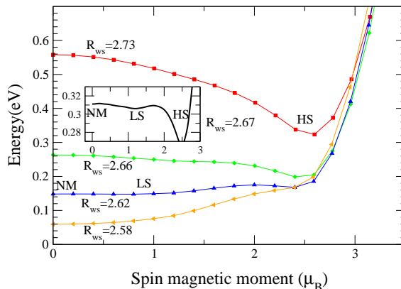
FIG. 3: Variation of the TBGGA total energy per atom with the magnetic moment (fixed spin moment calculation for the ferromagnetic state) for fcc Fe at several Wigner-Seitz radii R_{WS} in a.u.. Note the presence of stable (or metastable) non magnetic (NM), Low spin (LS) and High spin (HS) states which is clearly seen in the inset. The zero of energy is arbitrary.
