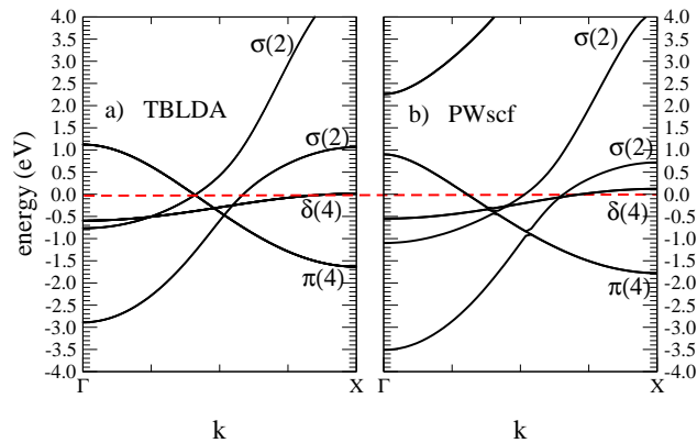
FIG. 9: a) TBLDA and b) PWscf band structure of a non-magnetic Fe monatomic wire with an interatomic distance of 4.29 a.u.. Each band is labelled by its symmetry character and degeneracy (including spin).
