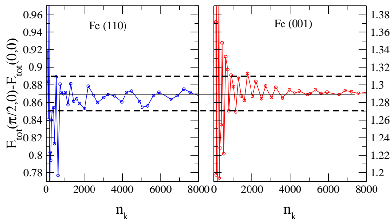
FIG. 7: Convergence of the magnetic anisotropy E_{tot}(\pi/2, 0) - E_{tot}(0, 0) with respect to the number of k points n_k in the first Brillouin zone, for (110) and (001) Fe bcc, unsupported monolayers. The magnetic anisotropy is oscillating around its asymptotic value (full straight line) with an amplitude below \pm 0.02 meV when n_k is larger than 1000.
