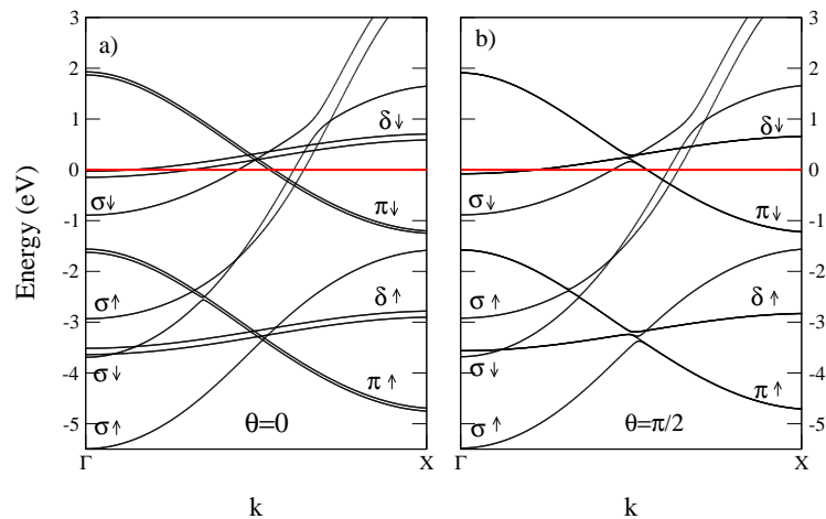
FIG. 11: TBLDA band structure including spin-orbit coupling for a magnetic Fe monatomic wire (interatomic distance d=4.16 a.u.) with a magnetization a) parallel and b) perpendicular to the wire.
