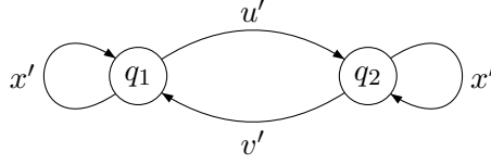
Figure 13: A configuration contained in \mathcal{A} .
