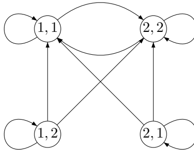
Figure 14: The graph G_2(\mathcal{A}) .
