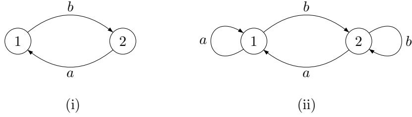
Figure 17: Two automata.
