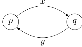
Figure 11: Forbidden configuration for \mathcal{R} -trivial automata.
