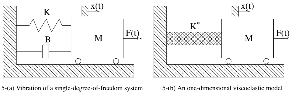
FIG. 5 – Viscous vs. viscoelastic systems
