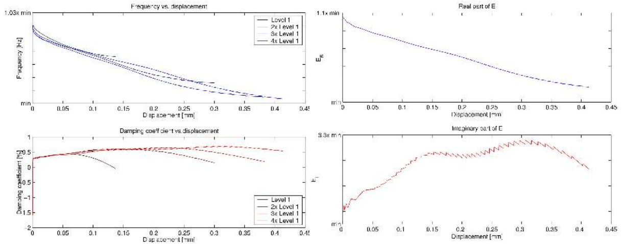
4-(a) Instantaneous Resonant frequency and Damping factor vs. displacement 4-(b) Instantaneous complex Young's modulus vs. displacement
