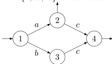
Figure 2.5: The minimal automaton of \{a, ac, bc\} .
