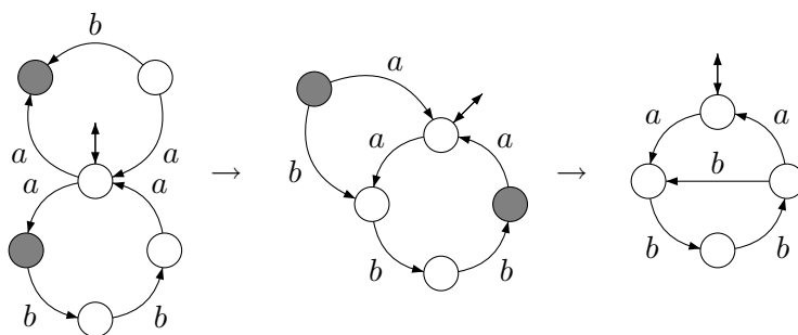
Figure 3.6: Construction of a reversible automaton accepting \langle \bar{a}ba, abba \rangle .
