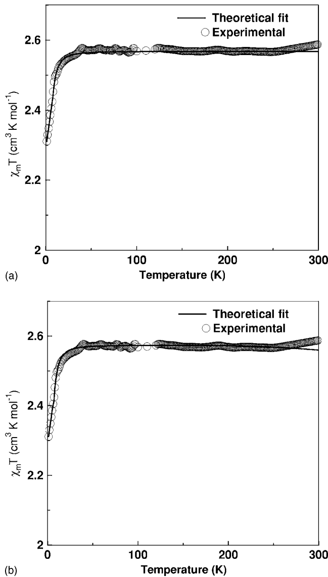
FIG. 4. Theoretical fit of temperature dependence of \chi_M T for (a) t=0.01 eV and (b) t=0.00065 eV. Error in the fit R calculated from R = \sum_i [\chi_{\text{expt}}(T_i) - \chi_{\text{calc}}(T_i)]^2 / \sum_i \chi_{\text{expt}}(T_i)^2 for (a) 1 \times 10^{-5} and (b) 1.35 \times 10^{-5} .
