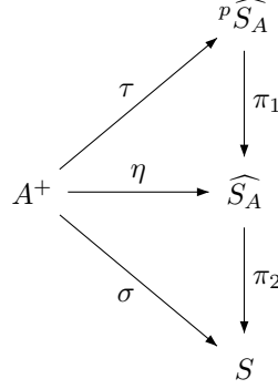
Figure 3.1: A commutative diagram.
