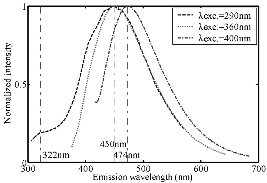
Figure 10: Normalized emission spectra of the resin cured in-situ for 18h at 100°C.
