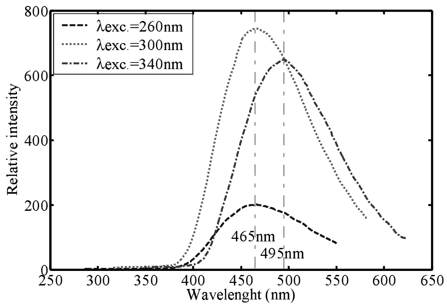
Figure 6: Low temperature phosphorescence spectra of ex-situ cured resin.
