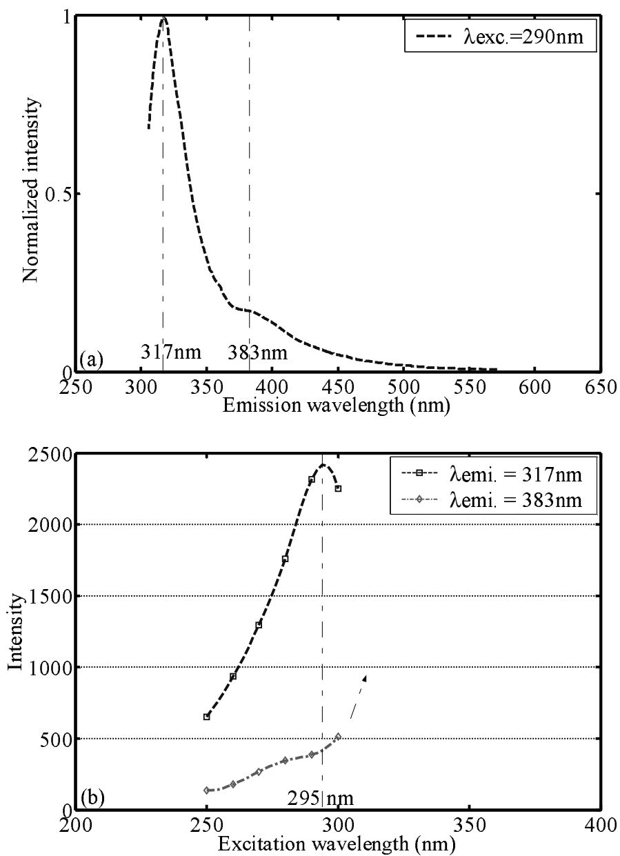
Figure 2: Room temperature photoluminescence spectra of the base resin. (a): Emission spectrum; (b): Excitation spectra
