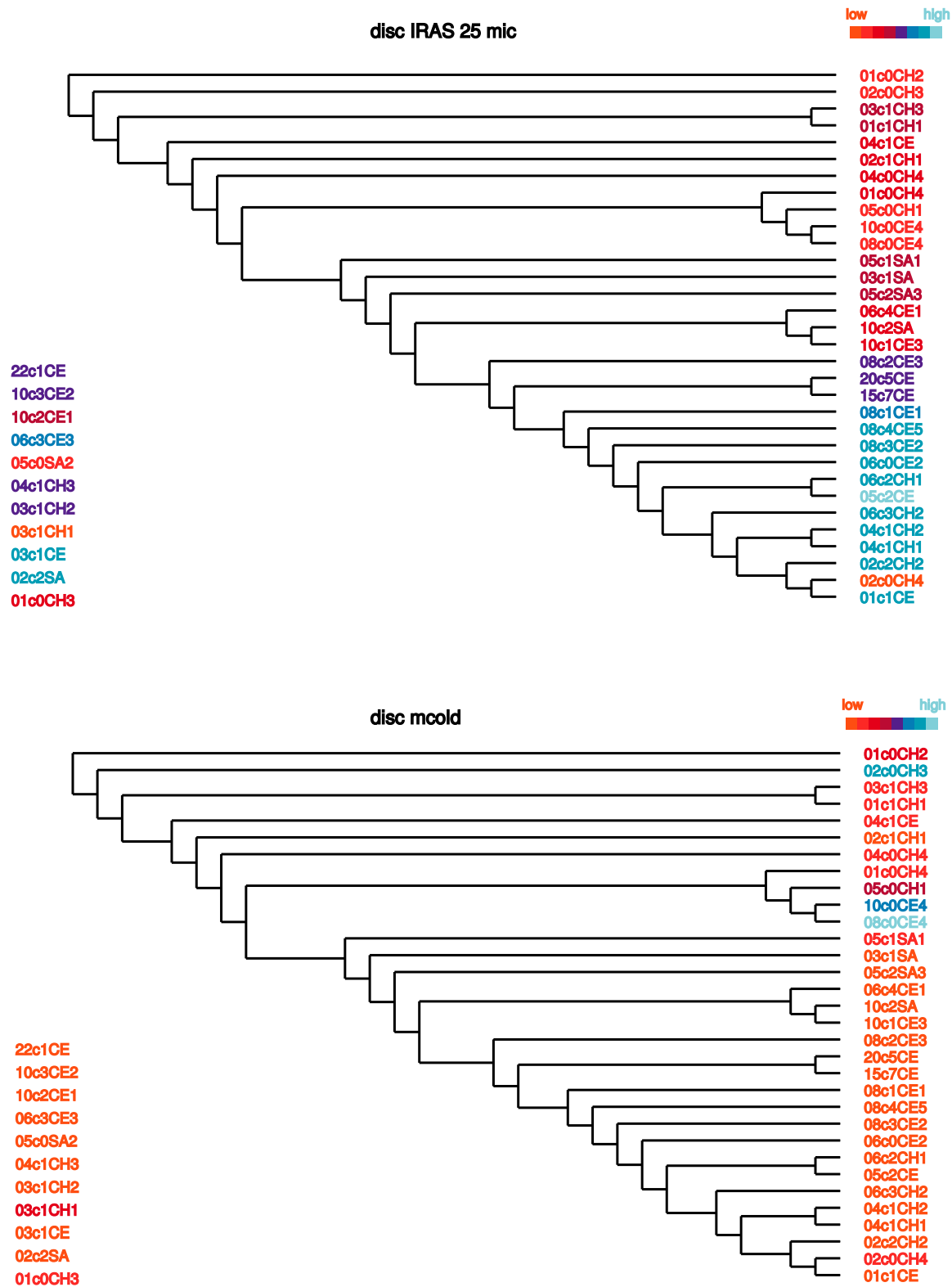
Fig. 4. Same as Fig. 3 for two disc characters.
