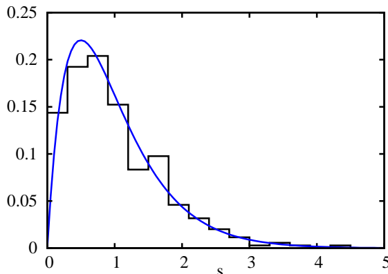
Figure 6. Experimental histogram of P(s) in the dressed cavity; Semi-Poisson law: P(s) = 4se^{-2s} (blue curve).
