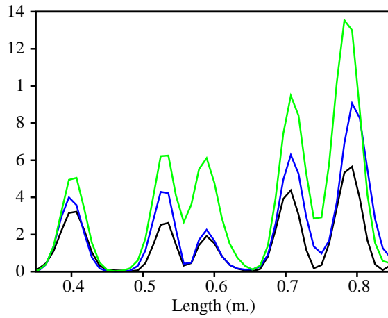
Figure 5. Scaling law in 1/k of the amplitudes of the peaks associated to the DOs. Gaussian normalized frequency windows with equal variances (2 GHz) centered on 10 GHz (green), 15 GHz (blue) and 20 GHz (black) were used. An excellent agreement with the prediction of formula (6) is observed.
