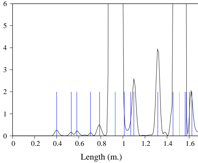
Figure 3. Zoom ( \times 10^4 ) of the length spectrum shown in Figure 1 on the length range from 0 to 1.6 m using an enlarged scale for the amplitude of the peaks : POs (green sticks), DOs (blue sticks)
