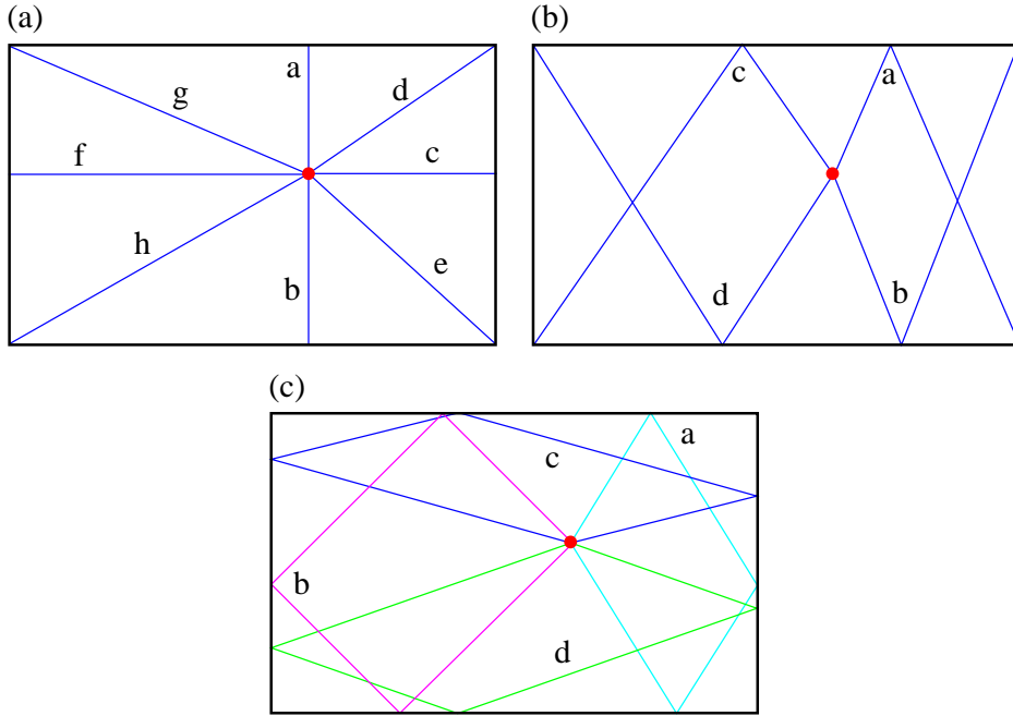
Figure 4. Three different kinds of one-diffraction event diffractive orbits associated to the position of the scatterer used numerically and experimentally: (a) direct self-retracing DOs (1st kind), (b) self-retracing DOs (2nd kind), (c) 3-bounce DOs (3rd kind).
