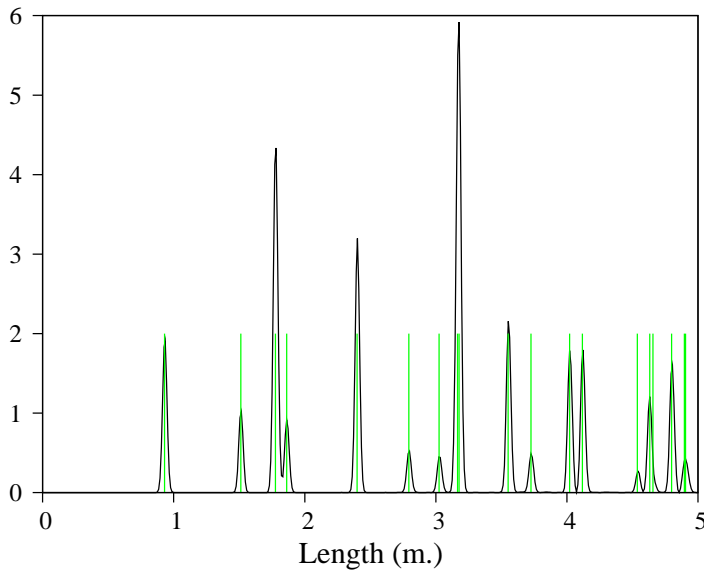
Figure 1. Length spectrum computed in a rectangular cavity with a single point scatterer. Approximately 11000 resonances have been used. Green sticks indicate the lengths of the POs listed in Table 1.
