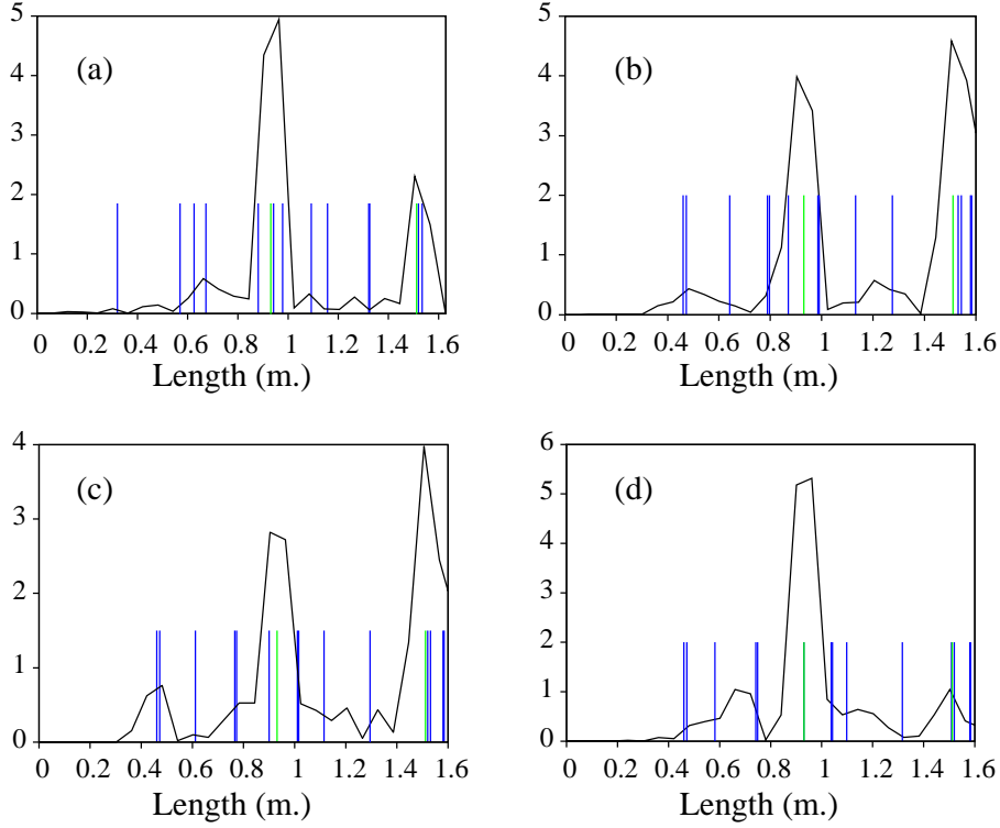
Figure 8. Experimental length spectrum for 4 different positions of the scatterer measured from the upper left corner of the rectangular cavity: (a) x = 28.5 cm, y = 13 cm, (b) x = 43.5 cm, y = 23 cm, (c) x = 45 cm, y = 23 cm, (d) x = 46.5 cm, y = 23 cm. The corresponding DOs of the three kinds are depicted by blue sticks. POs are indicated by green sticks.
