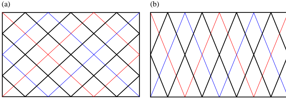
Figure 2. Periodic orbits representation with indices (a) (2,3) (b) (1,4). Continuous deformations of the orbit shown in thick black lines lead to the orbits shown in red or blue lines
