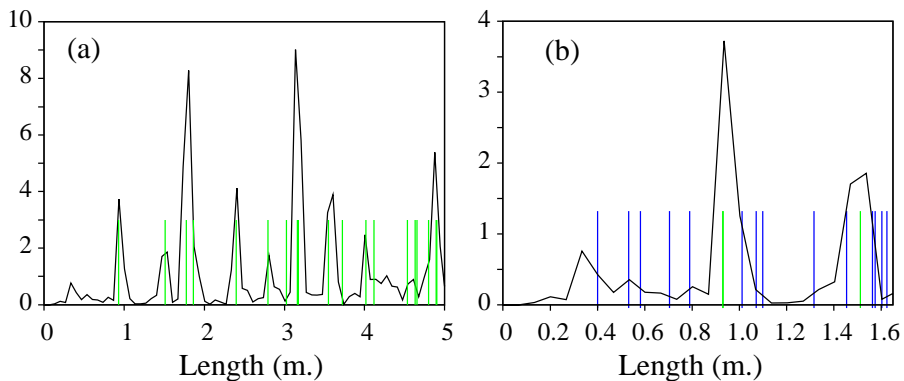
Figure 7. Experimental length spectrum computed from 300 actual resonances measured from 500 MHz to 5 GHz. The position of the center of the scatterer is the same as in the numerical results of the previous section. (a) length range from 0 to 5 m, POs indicated by green sticks; (b) length range from 0 to 1.6 m, POs indicated by green sticks, DOs by blue sticks.
