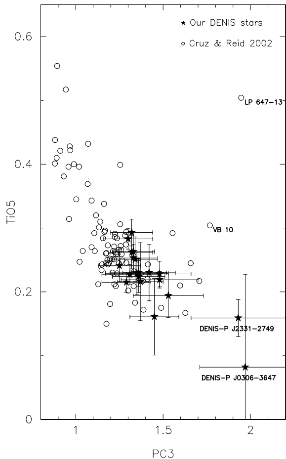
Fig. 4. TiO5 vs. PC3 diagram. The coolest stars are on the right side. The filled stars represent the 20 T152 measurements from this paper, and the empty circles represent measurements from Cruz & Reid (2002). LP 647-13 (M9.0), VB 10 (flare star, M 8.0), DENIS-P J0306-3647 and DENIS-P J2331-2749 (both M 8.5 at 11 pc) are individually identified. The error bars are determined from the flux fluctuations over the integration intervals, and therefore represent lower limits to the true uncertainty. (The NTT stars are not plotted).
