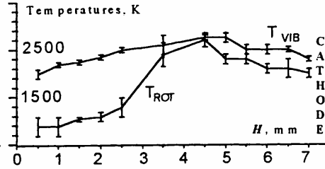
Figure 5. Axial distribution of T_{vib} and T_{rot}
