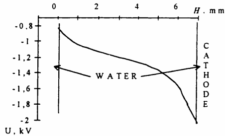
Figure 2. Plasma potential distribution
