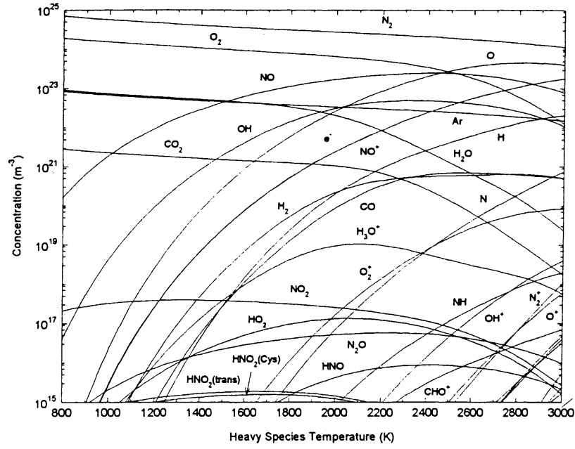
Figure 8. First zone : T_{tr e-} = T_{ex}^{at} = T_{ex}^{d at} = 3.5 T_{tr h} ; T_{vb} = 2 T_{tr h} ; T_{rot} = T_{tr h}
