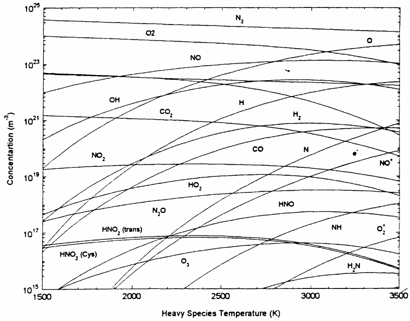
Figure 9. Second zone : T_{vb} = T_{tr h} ; T_{rot} = T_{tr h} ; T_{tr e-} = T_{ex}^{at} = T_{ex}^{d at} = 1.5 T_{tr h}
