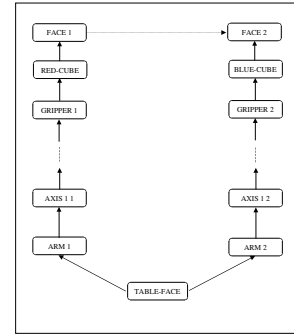
FIGURE 3. Kinematics inversion example using two Stäubli Rx90 arms and the corresponding kinematic graph.
