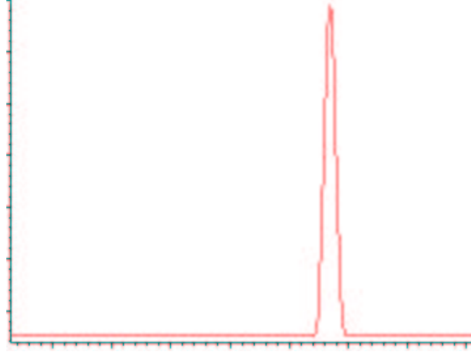
FIGURE 3. Distribution over the angle: P(\theta \mid o_k)
