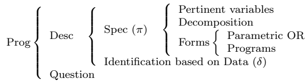
Figure 2: Structure of a bayesian program.
