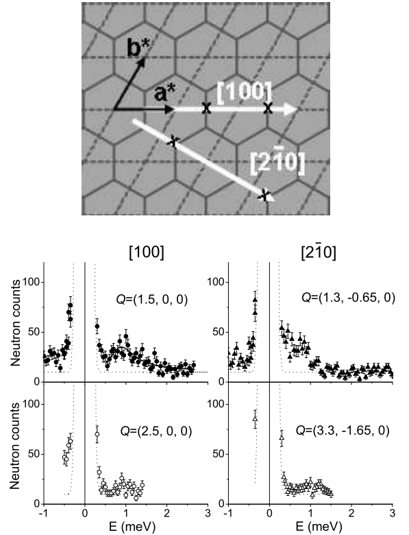
FIG. 1: Top : Intersection of the Brillouin zones with the (a^*, b^*) scattering plane (dark gray lines). The white arrows indicate the Q -scans performed in both the [100] and [2\bar{1}0] directions. Bottom : E-scans at 2 K for two different Q positions in each direction (crosses in the top panel). The thin lines are Gaussian fits of the incoherent peak. The thick line is a lorentzian fit (see text).
