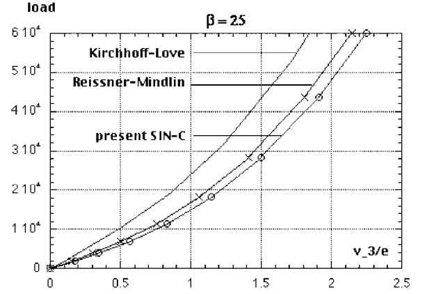
Fig. 4. Transverse displacement v_3(a/2, a/2, 0) of a simply supported square sandwich plate with \beta = 25 : comparison of different plate models.
