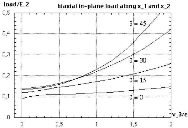
Fig. 9. Four layer (\theta, -\theta)_s simply supported square panel under biaxial in-plane load: angle orientation and post-buckling response.
