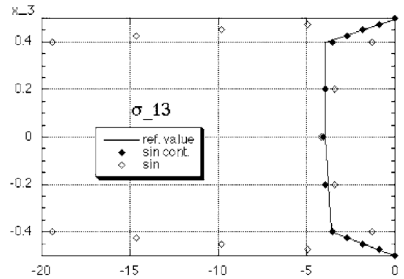
Fig. 2. Distribution of \sigma_{13}(0, a/2, z) with respect to the thickness co-ordinate.
