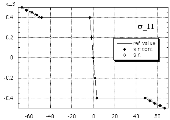
Fig. 1. Distribution of \sigma_{11}(a/2, a/2, z) with respect to the thickness co-ordinate.
