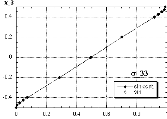
Fig. 3. Distribution of \sigma_{33}(a/2, a/2, z) with respect to the thickness coordinate.
