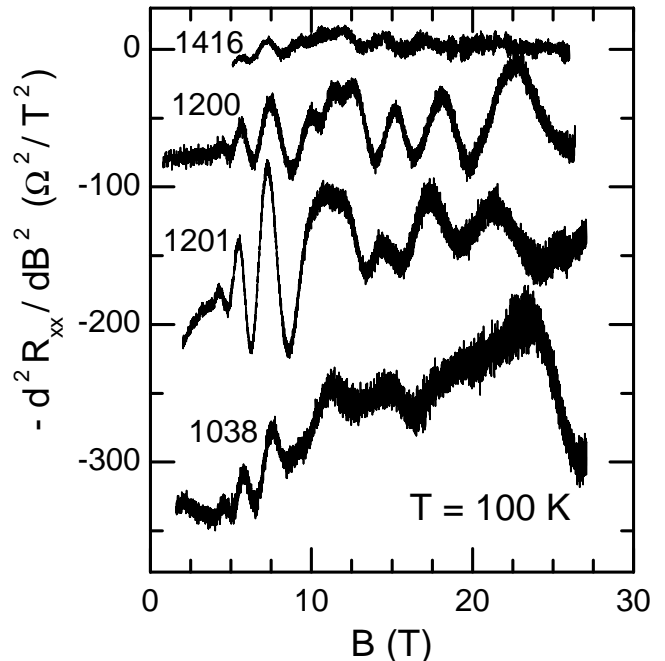
FIG. 1: Second derivative of the longitudinal resistance versus magnetic field measured at \theta = 0 and T = 100 K for the four samples investigated. Curves have been shifted vertically for clarity
