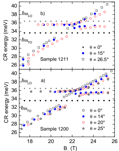
FIG. 2: Observed cyclotron energies for sample 1200 (a) and sample 1211 (b) for different tilt angles. The crosses and black down triangles are the measured LO and TO energies respectively and the empty squares the cyclotron energies in the PF configuration. Other points are the observed CR energies in the TF configuration: (a) full dots : \theta = 14^\circ , empty dots : \theta = 20^\circ , stars : \theta = 25^\circ and (b) full dots : \theta = 15^\circ , empty dots : \theta = 26.5^\circ . Results in (b) for B_\perp lower than 18 T correspond to filling factors > 2 when non parabolicity effects are apparent.
