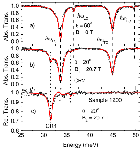
FIG. 1: Experimental transmission spectra (empty dots) of sample 1200. a) absolute transmission for B = 0 T and \theta = 60^\circ ; b) and c) absolute transmission and relative transmission respectively for B_\perp = 20.7 T and \theta = 20^\circ . The continuous red curves are the fit of data with the model described in the text.
