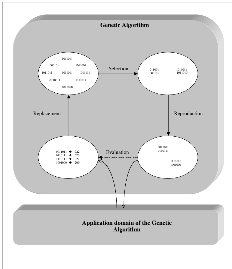
Figure 3: Genetic Algorithm iterations.
