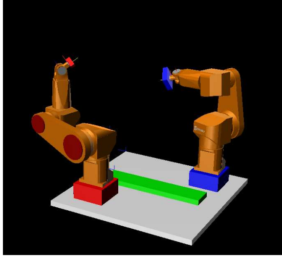
Figure 6: Kinematics inversion example using two Stäubli Rx90 arms.
