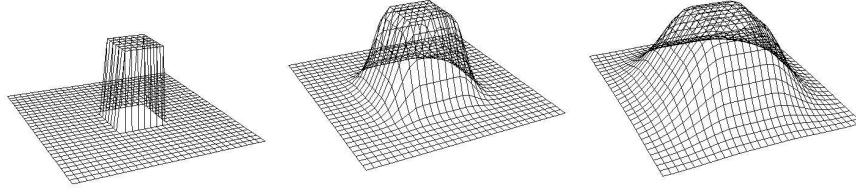
Figure 4: The distribution corresponding to inequality constraints induced by a Point-On-Face relationship for a square face at different values of temperature. The left figure shows the original constraints ( T = 0 ), while the middle and the right ones show these constraints relaxed at ( T = 50 ) and ( T = 100 ) respectively.
