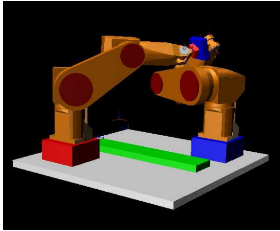
Figure 8: The solution obtained by the system.
