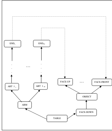
Figure 12: The kinematic graph for the calibration problem.
