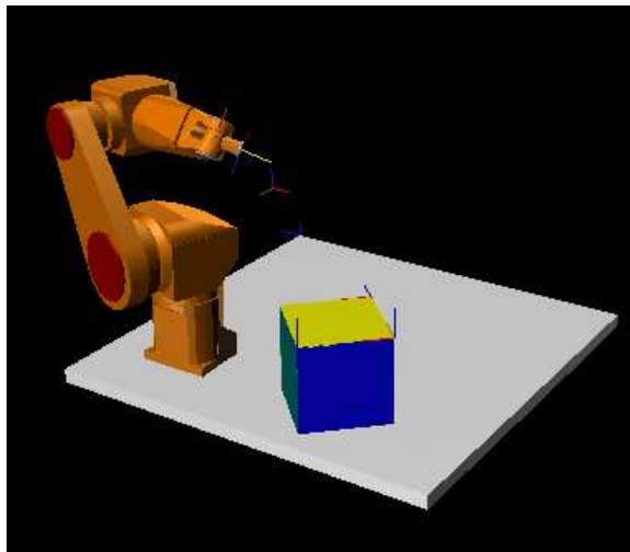
Figure 9: A parallelepiped pose and dimensions calibration problem using contact relationships.
