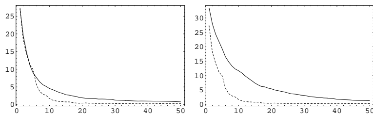
Figure 5: left: true target pdf; right: adaptive proposal density.
