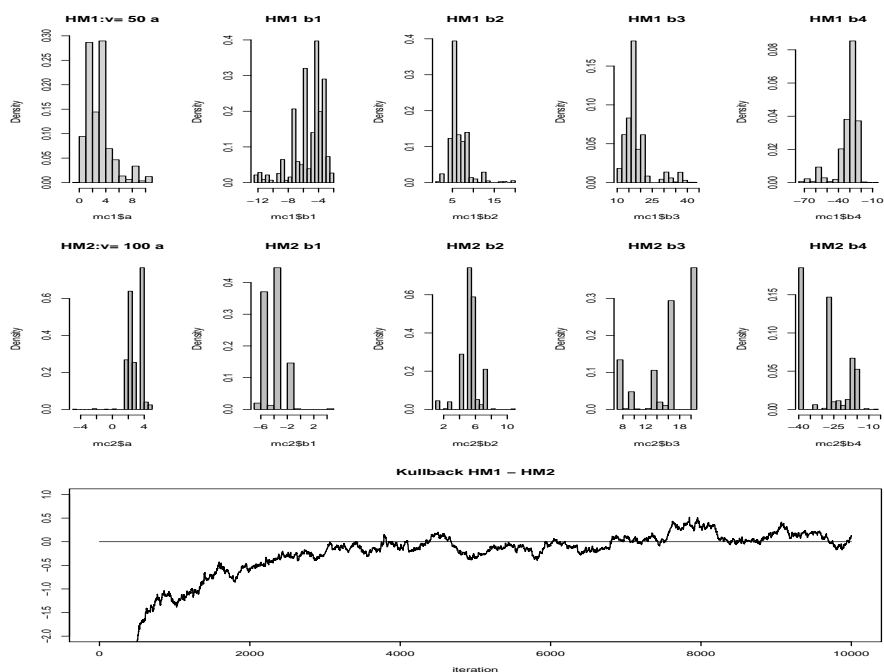
Figure 7: MH for the Logit model, n = 10,000 iterations; marginals from 1 chain and v_1 = 50 (row 1) against v_2 = 100 (row 2); bottom: D_N(p_1^n, p_2^n, f) based on N = 100 chains.
