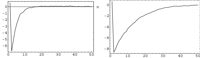
Figure 3: Plots of the difference n \mapsto D(p_1^n, p_2^n, f) for the IS with a gaussian proposal q_i = \mathcal{N}(0, \sigma_i^2) . Left: \sigma_1 = 3 vs. \sigma_2 = 30 ; Right: \sigma_1 = 3 vs. \sigma_2 = 100 .
