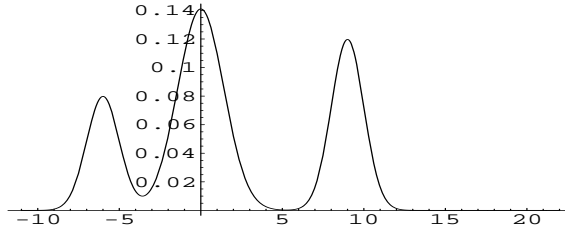
Figure 1: True mixture density (29).
