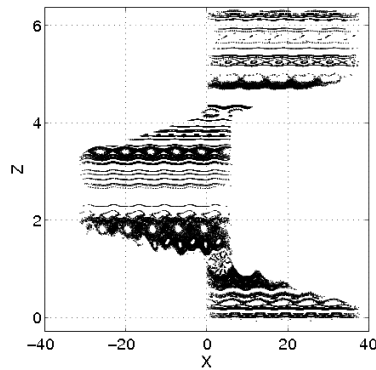
Fig. 6. Poincaré section of magnetic field lines.
