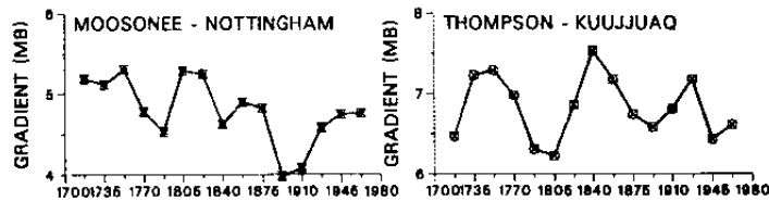
FIGURE 7. Trends of the reconstructed temperatures and SLP series: the means are computed over 35-year intervals by steps of 17.5 years. At the bottom, differences between SLP of extreme latitude (Moosonee and Nottingham Island) and extreme longitude (Thompson and Kuujuaq) are drawn.
