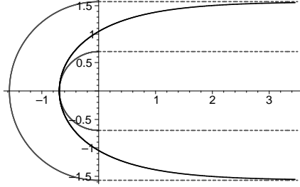
FIGURE 1. Les ouverts \mathcal{B}_{\ln(2)} \subset \Delta \subset \mathcal{B}_{\frac{\pi}{2}} .
