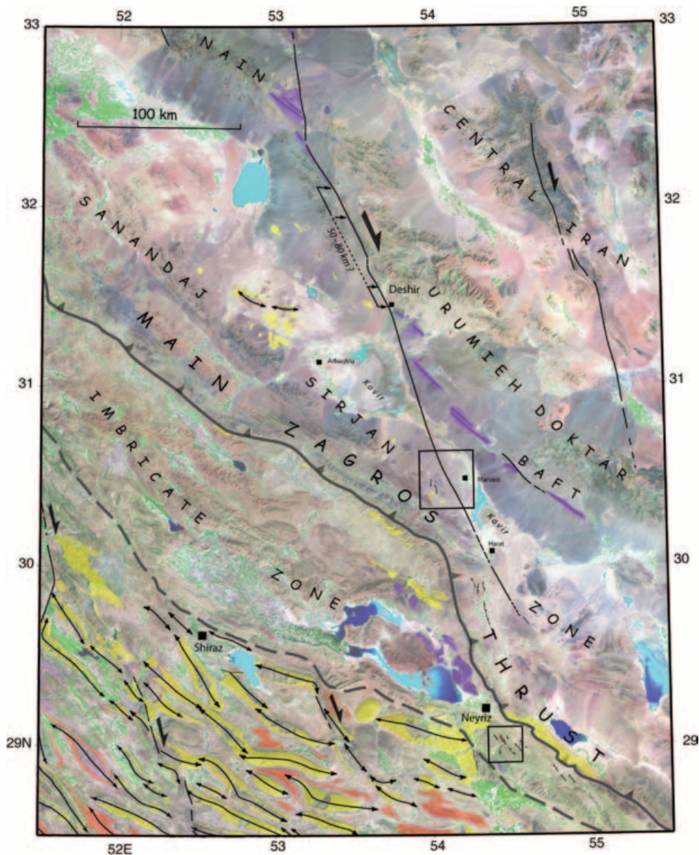
Figure 2. Landsat Mosaic of the Deshir Fault and surroundings. Geological information is adapted from Geological Survey of Iran (1985). The Main Zagros Thrust (MZT) that separates the Iranian Plateau from the Zagros Mountains indicates the suture between Central Iran and the former margin of Arabia. Thick dashed line indicates the transition between the imbricate zone and the Simply Folded Belt of Zagros. Ophiolites (in purple) outcrop both to the south (Neyriz ophiolites) and to the north (Urumieh-Oktar sequence) of the MZT. Lower Miocene neritic limestones (in yellow, Qom and Asmari-Jahrom formations, respectively, on the plateau and within the Zagros) are unconformable on the ophiolites. The neritic limestone and the Upper Miocene sandstones and microconglomerates of Agha Jari formation (in orange) outline the structure of the folded Zagros. The Deshir Fault cuts across the overall structure and morphology of the plateau and vanishes north of a prominent bend of the MZT. Normal faults are encountered west of and close to the southern termination of the Deshir Fault. Boxes indicate locations of Figs 3 and 6.
