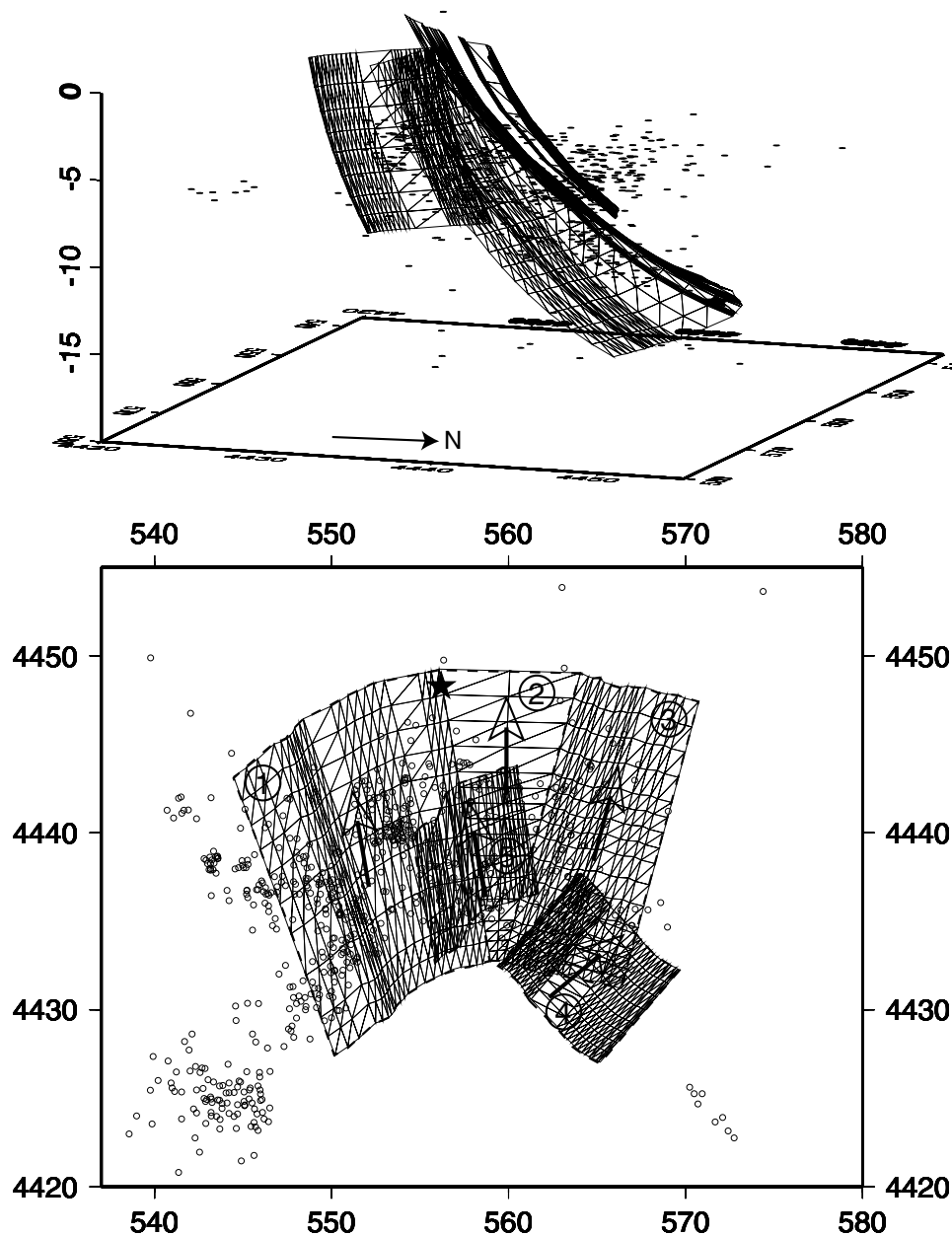
Figure 4. Fault plane model composed of 1572 triangular elements. The aftershocks and the location of the main shock (star) from Hatzfeld et al. (1997) are shown. Top, 3-D view from the northeast; bottom, map view; the arrows correspond to the slip azimuth and the numbers to the subfaults described in Table 2.
