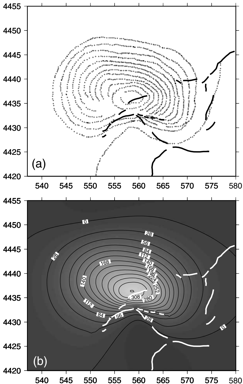
Figure 3. Digitized fringes (a) subsequently interpolated on a regular grid and (b) with the faults drawn for the 12219–22583 interferogram. The numbers correspond to the range change in mm in the ground-to-satellite line of sight.
