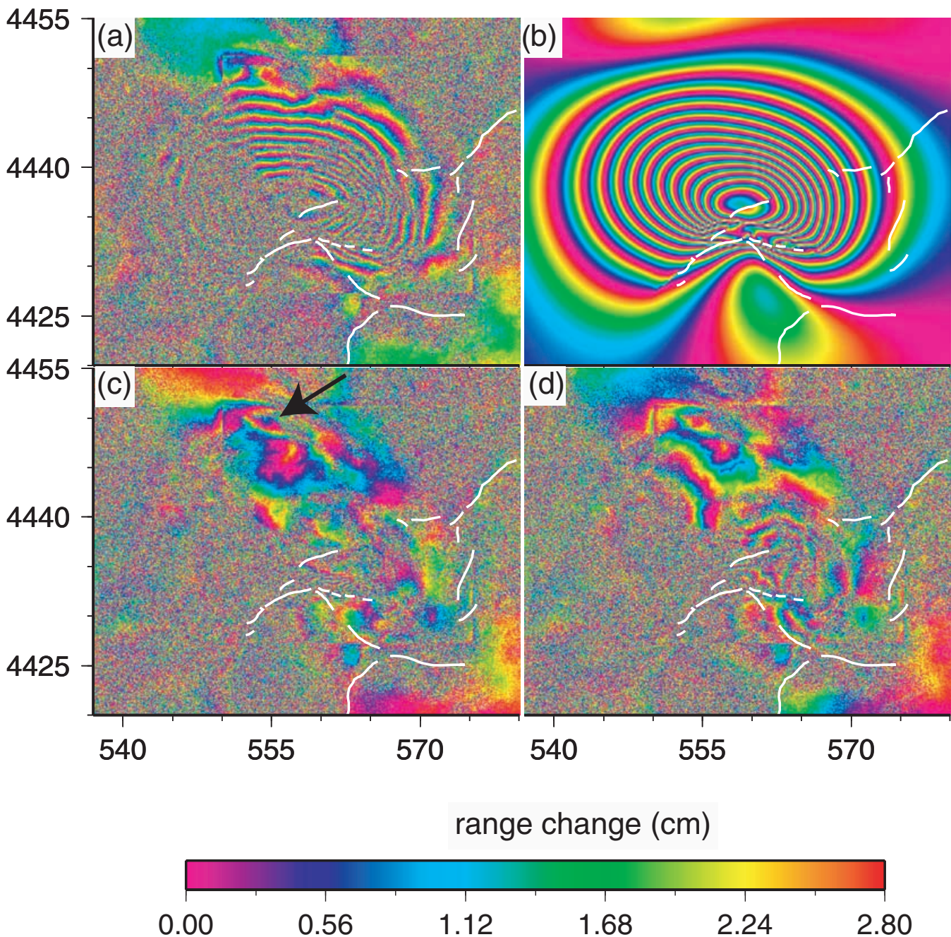
Figure 6. 12219–22583 interferogram: (a) observed and (b) synthetic interferogram obtained from the averaged co-seismic model; (c) residual interferogram obtained by removing (b) from (a)—the arrow indicates the location of a hypothetical antithetic fault (see text for details); (d) residual interferogram obtained by removing the model of Meyer et al. (1996) from (a).
