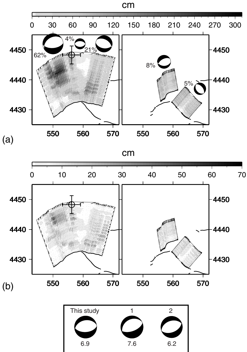
Figure 5. Averaged co-seismic slip distribution model (a) and corresponding standard deviation (b). Focal mechanisms for each subfault are shown. The composite focal mechanism is compared with (1) the Harvard CMT determination and (2) that obtained by Hatzfeld et al. (1997), the seismic moment M_0 ( 10^{18} N m) being indicated below.
