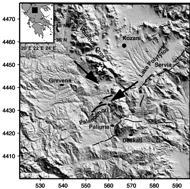
Figure 1. Location map of the 1995 Kozani–Grevena earthquake on a Digital Elevation Model (DEM) built with stereometric SPOT scenes. The star locates the epicentre of the main shock (Hatzfeld et al. 1997). The active normal faults are drawn in thin black lines and the thick lines correspond to the faults where surface breaks were observed after the quake (from Meyer et al. 1996). The arrows denote artefact areas of the DEM.
