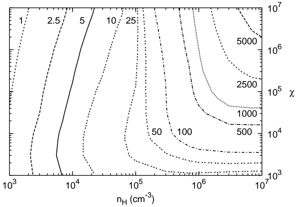
Fig. 26.— Intensity of the 1-0 S(1) H 2 transition in 10^{-6} \text{erg s}^{-1} \text{cm}^{-2} \text{sr}^{-1} assuming a face on geometry.
