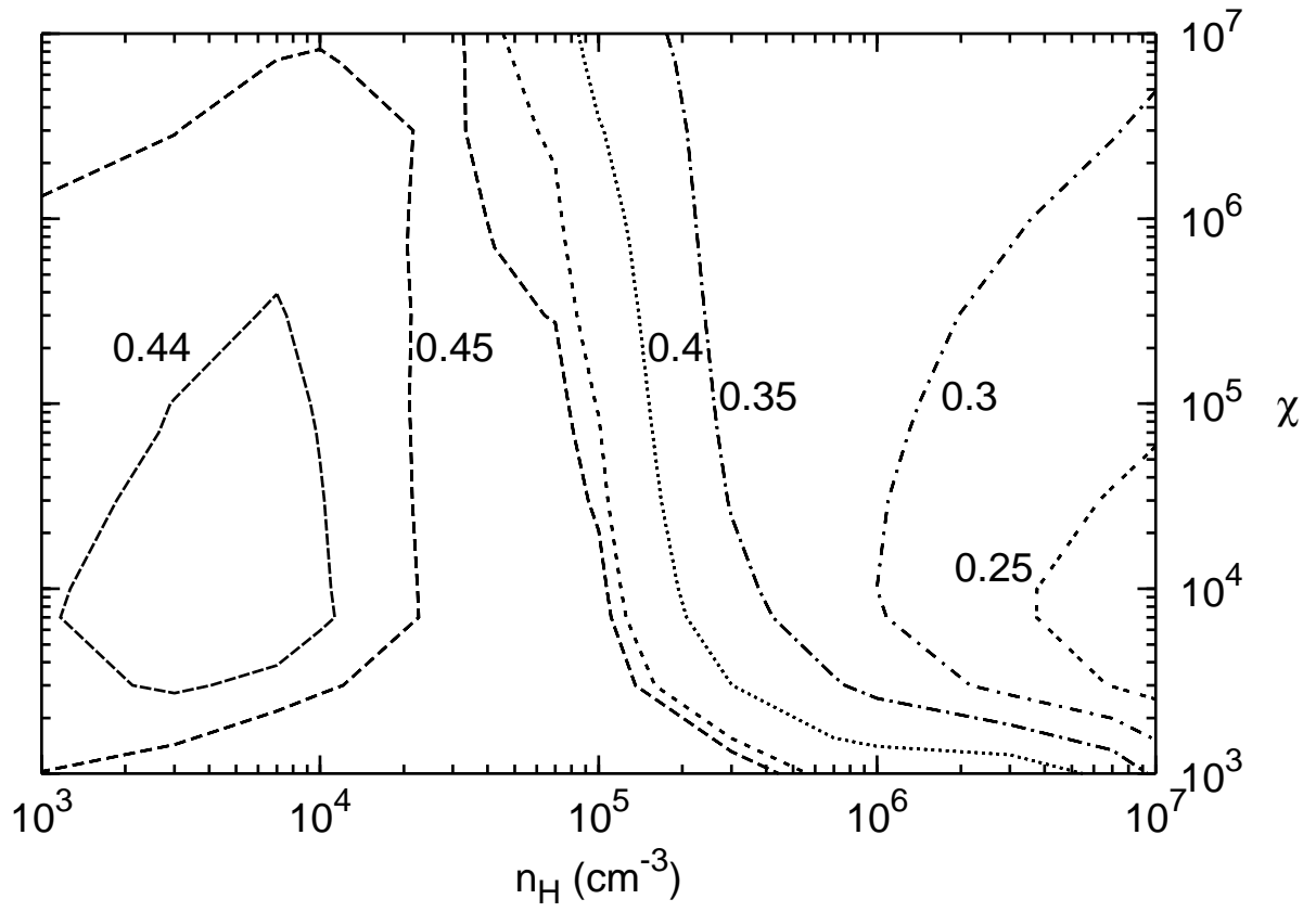
Fig. 29.— Ratio of the intensities of the \text{H}_2 lines 1-0 S(2)/1-0 S(1) given by the models.
