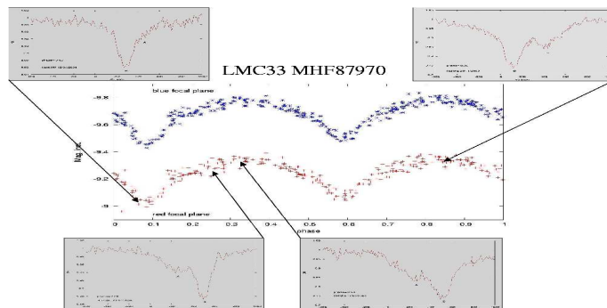
Figure 1. Binary LMC33-MHF87970, P=7.117d , MACHO60.7950.16. The central panel shows the MACHO lightcurves in phase. The four little panels show the GIRAFFE spectra and their correspondence with the phases.
