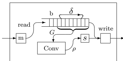
Figure 6: Description of the encoder component.
