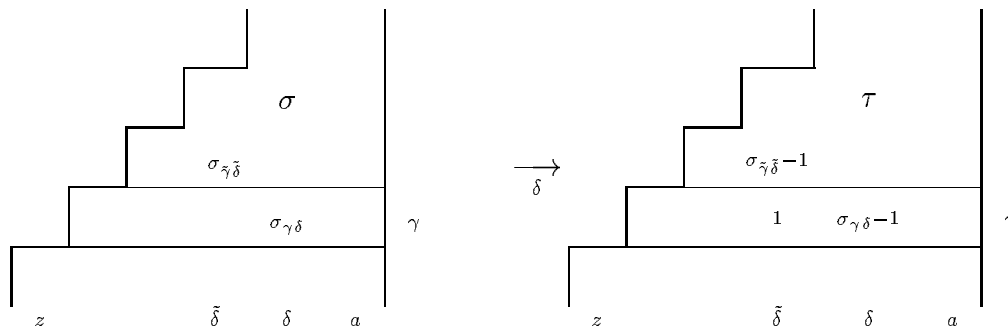
Figure 4: How Rule 2 _{\tilde{\delta}} works.
