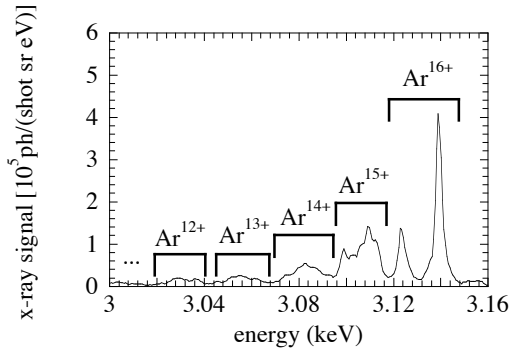
FIG. 2: K-shell x-ray spectrum of 350 Å average radius Argon clusters irradiated by 500 fs FWHM and 3.0 mJ laser pulses, corresponding to 1.6 \times 10^{16} W/cm 2 maximum intensity. Different lines are emitted from different charge state ions, up to Ar 16+ .
