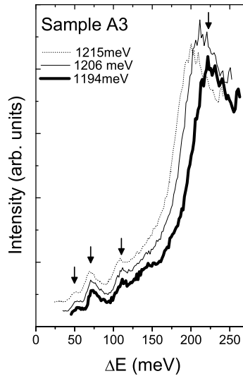
FIG. 1: Normalized PLE spectra of the A3 sample taken at 4 K for E_{det}=1194, 1206 and 1215 meV, where \Delta E = E_{exc} - E_{det} .
