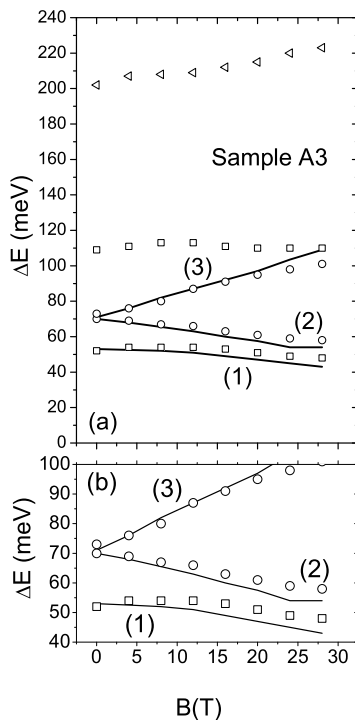
FIG. 4: Magnetic field dispersion of PLE resonances in sample A3 in open figures with the calculated energy transitions in solid lines (a) and a zoom (b) of the polaron states (1), (2) and (3). See Section IV for details and parameters of the calculated fit.
