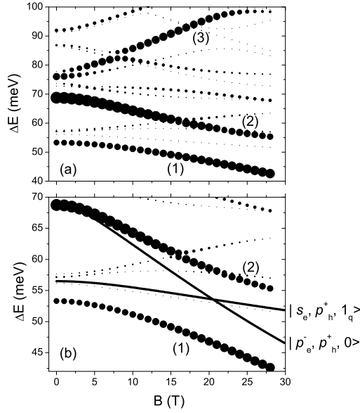
FIG. 5: Calculated excitonic polaron energies and intensities as a function of the magnetic field (a) and a zoom (b) of the anticrossing between polaron states (1) and (2). The solid lines in (b) correspond to noninteracting exciton-phonon states. The area of the circles are proportional to the oscillator strengths.
