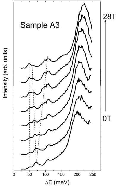
FIG. 2: Magneto-PLC spectra of the A3 sample recorded at 4 K from B=0 to B=28 T every 4 T and for a E_{det}=1215 meV. Traces have been vertically offset for clarity. The dashed lines are guides for the eyes.
