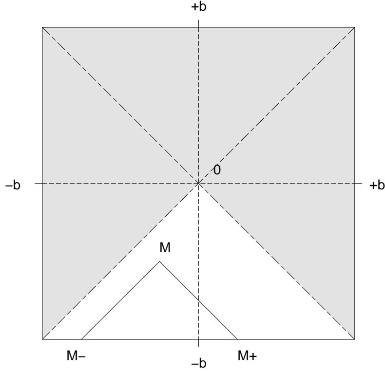
Figure 1: Triangle \Delta_M .
