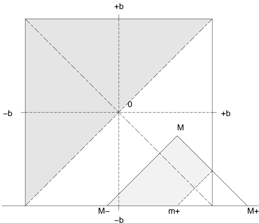
Figure 2: Triangle \Delta_M and (Mm_+M_-) .
