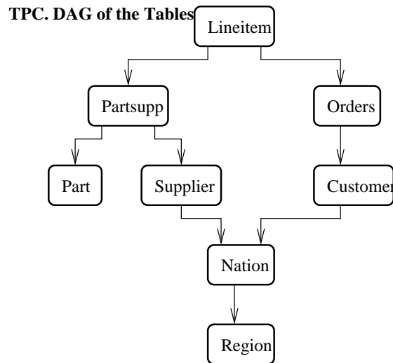
Figure 1: The dag of the relations of the TPC
