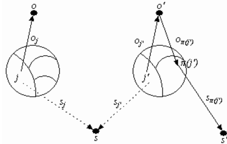
Figure 4: Reassigning the clients in N_S(s) \cup N_{S^*}(o)
