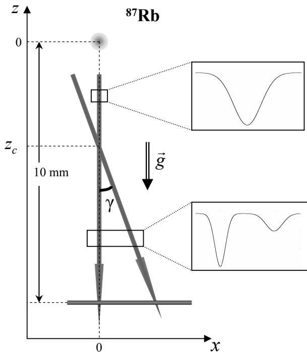
FIG. 1: Schematic view of the guiding setup. The initial ^{87}\text{Rb} cloud is shown at the altitude z = 0 . When the magneto-optic trap is switched off, a vertical laser beam is switched on and the cloud, partially trapped by the associated dipole force, falls in the gravity field. At time t_0 a second oblique guide is switched on. The two guides cross at the altitude z_c and form an angle \gamma . The trapping potential seen by the atoms at two different altitudes is shown in the insets. Finally, the atoms are probed 1 cm below the initial position.
