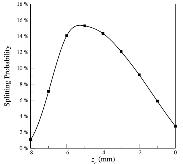
FIG. 7: Total splitting efficiency P_s [Eq.(22)] as a function of the crossing altitude z_c of the laser beams. This probability has been averaged over the initial conditions chosen for z_0 and \dot{z}_0 , and summed over v_0 . The size of the initial atomic cloud is \sigma_0 = 0.30 mm. All other parameters are as in Figure 6.
