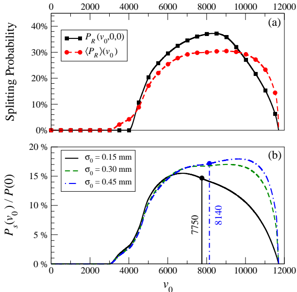
FIG. 6: (Color online) State-dependent splitting efficiency as a function of the initial level v_0 . Upper graph (a): the probability P_R(v_0, 0, 0) of finding the atom in the oblique guide at the end of the propagation is shown as a black solid line for the initial condition z_0 = \dot{z}_0 = 0 . The same probability averaged over z_0 and \dot{z}_0 , \langle P_R \rangle(v_0) , is shown as a red dashed line. Lower graph (b): The averaged splitting probability P_s(v_0) scaled by the same factor P(0) as in Figure 4 is shown as a function of v_0 for various sizes of the atomic cloud \sigma_0 and for T_0 = 14 \mu\text{K} . The cloud sizes \sigma_0 = 0.15, 0.30 and 0.45 mm correspond to the solid black, dashed green and dash-dotted blue curves respectively. These probabilities have been averaged over the initial classical conditions chosen for z_0 and \dot{z}_0 . The guide parameters are as in Figure 5. The two vertical lines indicate the average value of v_0 in the oblique guide for \sigma_0 = 0.15 mm (black solid line), \langle v_0 \rangle = 7750 , and \sigma_0 = 0.45 mm (blue dash-dotted line), \langle v_0 \rangle = 8140 .
