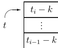
Figure 6: Snapshot of column-bumping process for Lemma 5.2.
