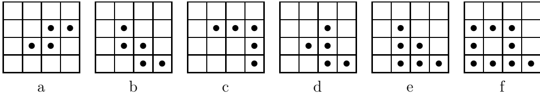
Figure 1: Several examples and counter-examples for the Definition 5.1 of ribbons.
