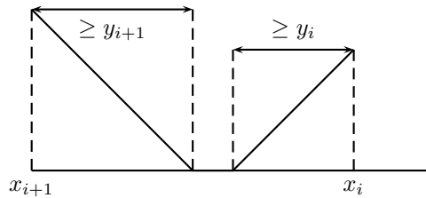
FIGURE 7. If the i^{\text{th}} peak is of type 0 and the (i+1)^{\text{st}} peak is of type 1, we have x_i - x_{i+1} \geq y_i + y_{i+1} .
