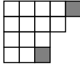
FIGURE 1. Ferrers diagram of the overpartition \lambda = (\overline{5}, 4, 3, \overline{3}) of weight 15.
